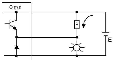
Source type transistor output
