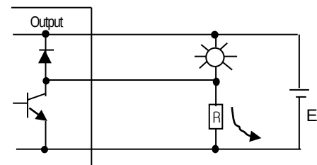
Sink type transistor output
